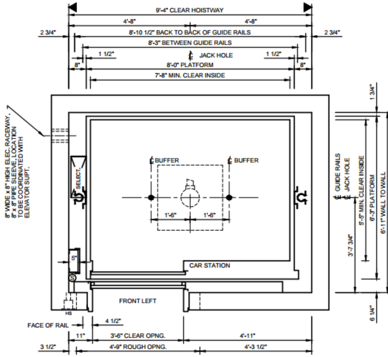
A HOISTWAY PLAN
