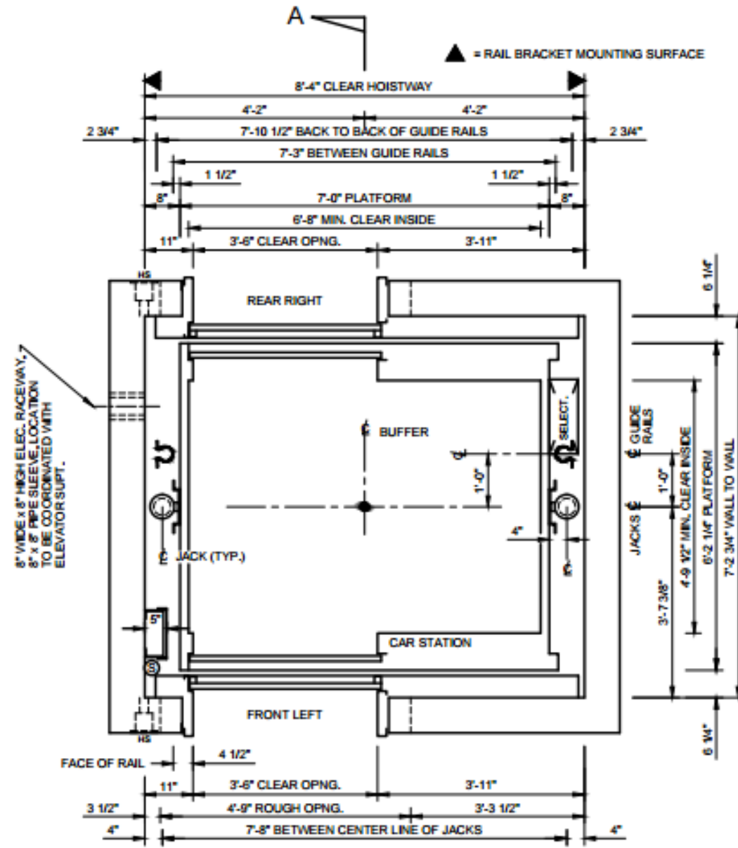
A HOISTWAY PLAN
