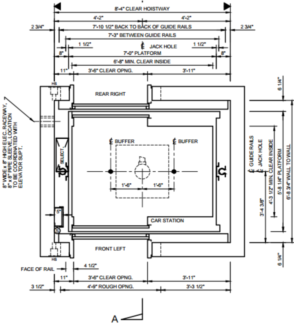
HOISTWAY PLAN
