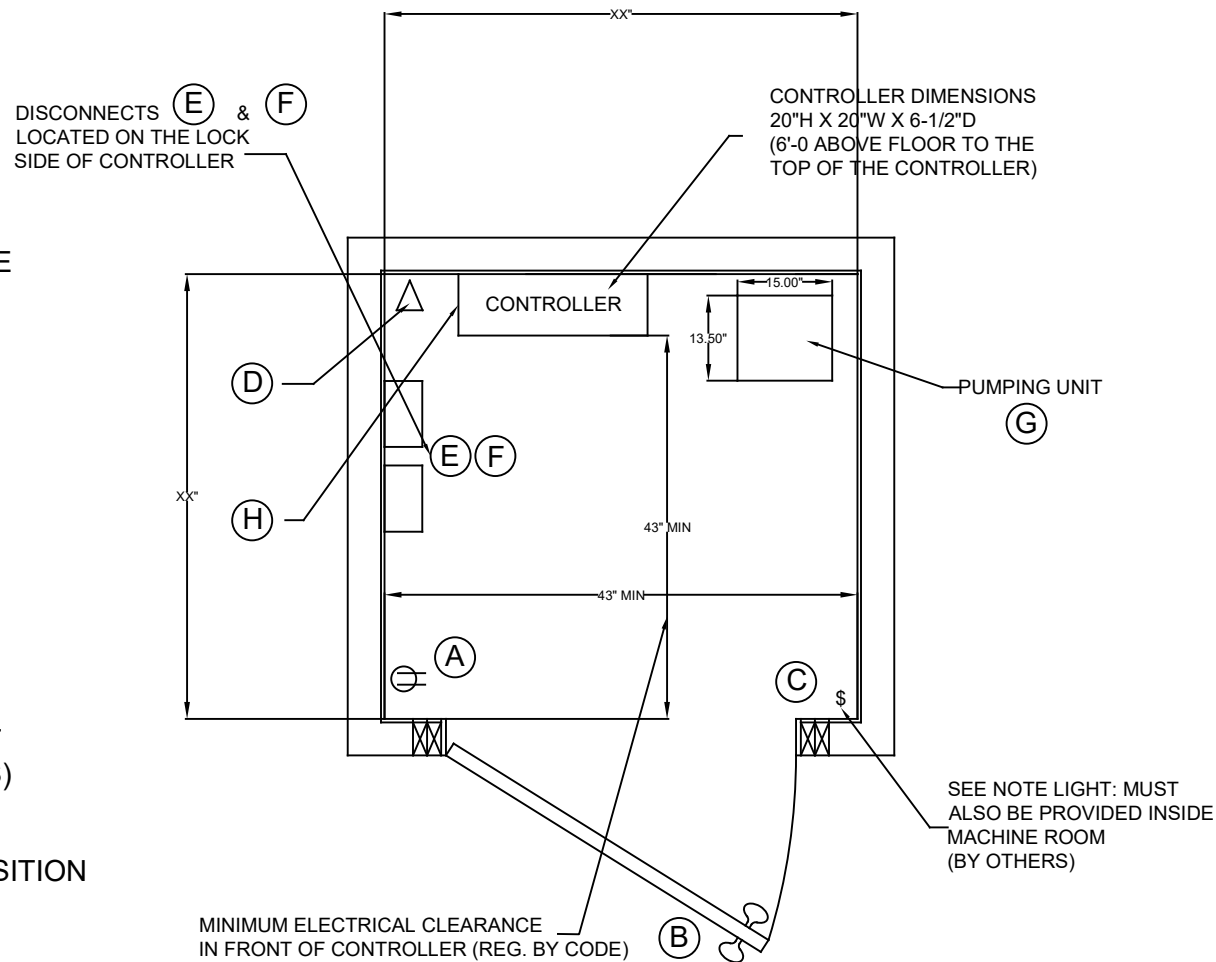
MACHINE ROOM PLAN VIEW SCALE= NOT TO SCALE
