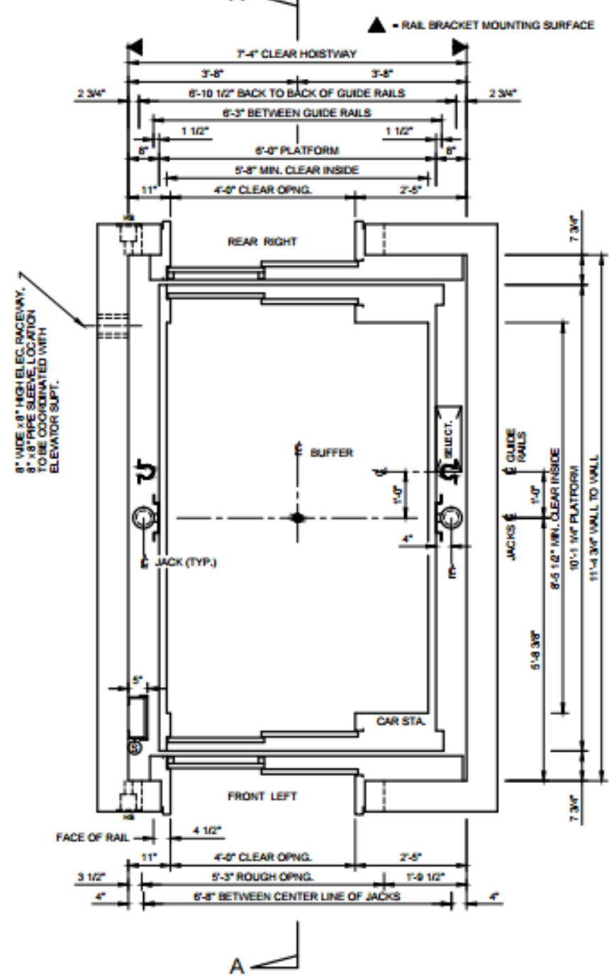
A HOISTWAY PLAN
