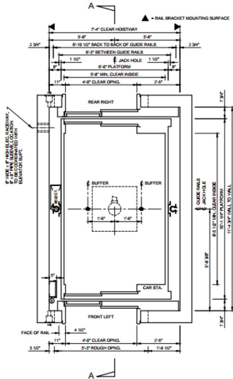
HOISTWAY PLAN
