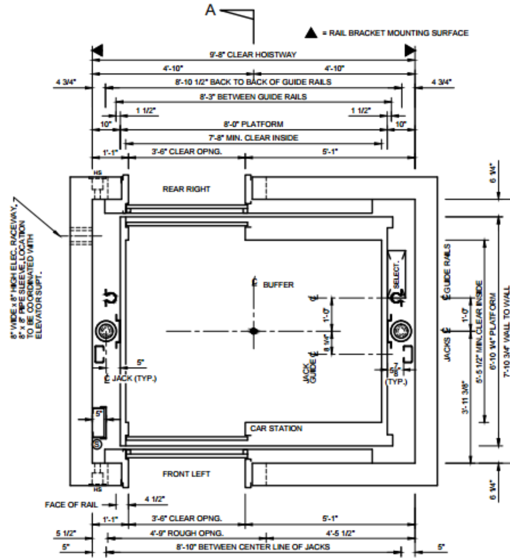
A HOISTWAY PLAN
