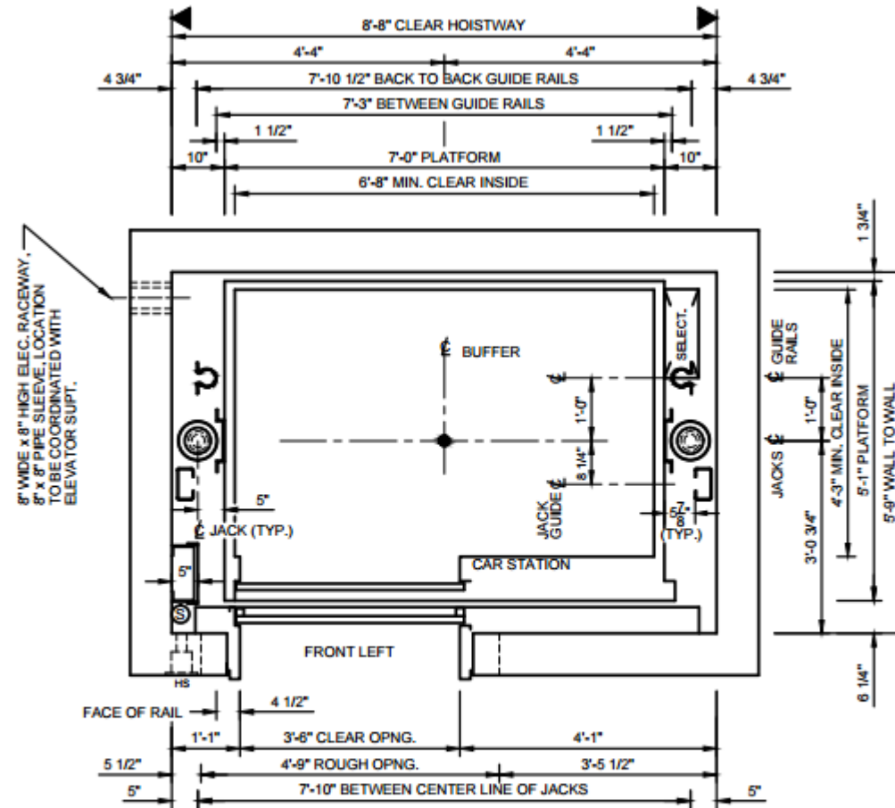
A HOISTWAY PLAN
